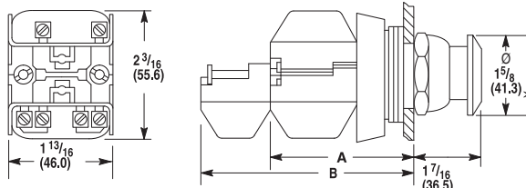
Mushroom Head — Maintained and Momentary
