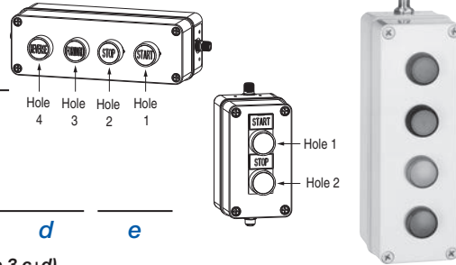
4-Hole Assembled Station Cat. No. 800F-VHA3A4J3J4J
