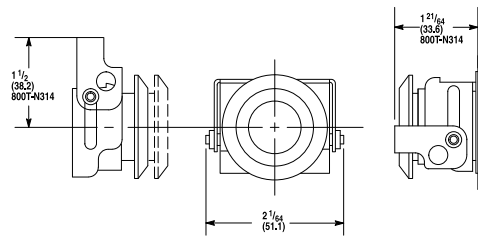
Push-Pull/Twist Padlocking Attachment
