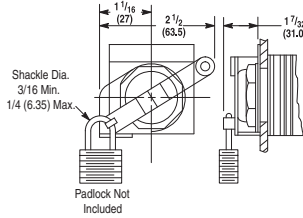
Locking Attachment for Extended, Non-Illuminated Push Buttons
